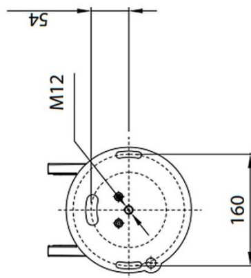
Mount Bottom Plate
